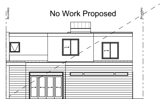
West Elevation 1:200
